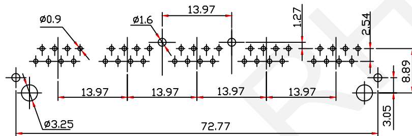
PCB Layout
